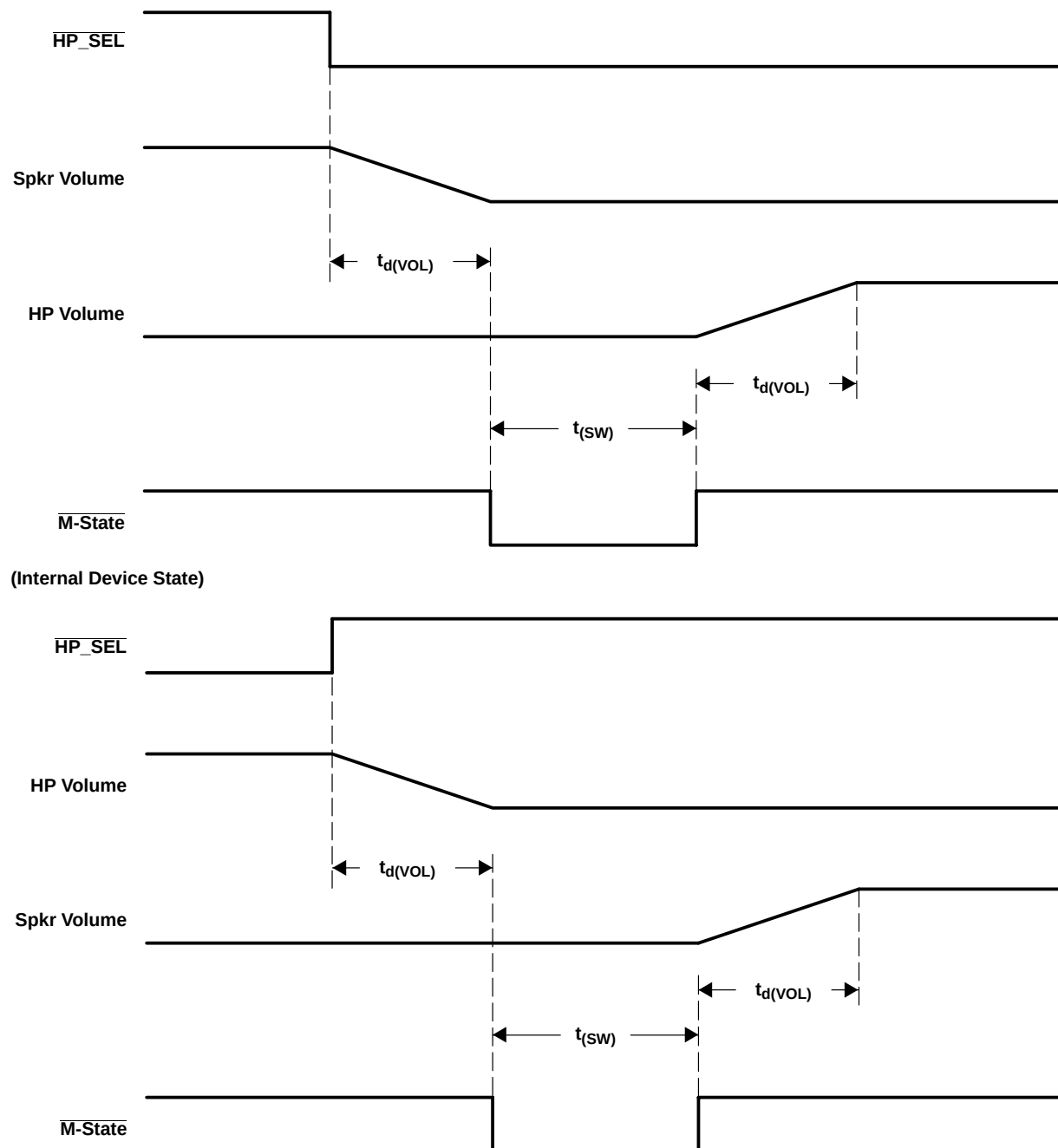
Figure 3-8. \overline{\text{HP\_SEL}} Timing
